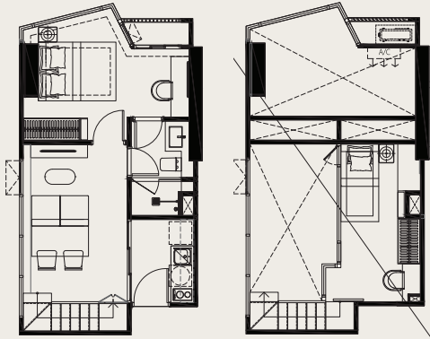
D-BP1-01, D-BP1-01M 34.63 - 34.69 SQ.M
