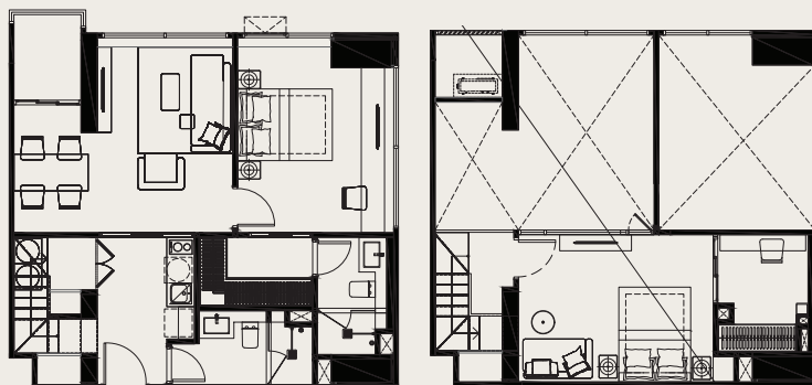
D-BP4-01 58.24 SQ.M
